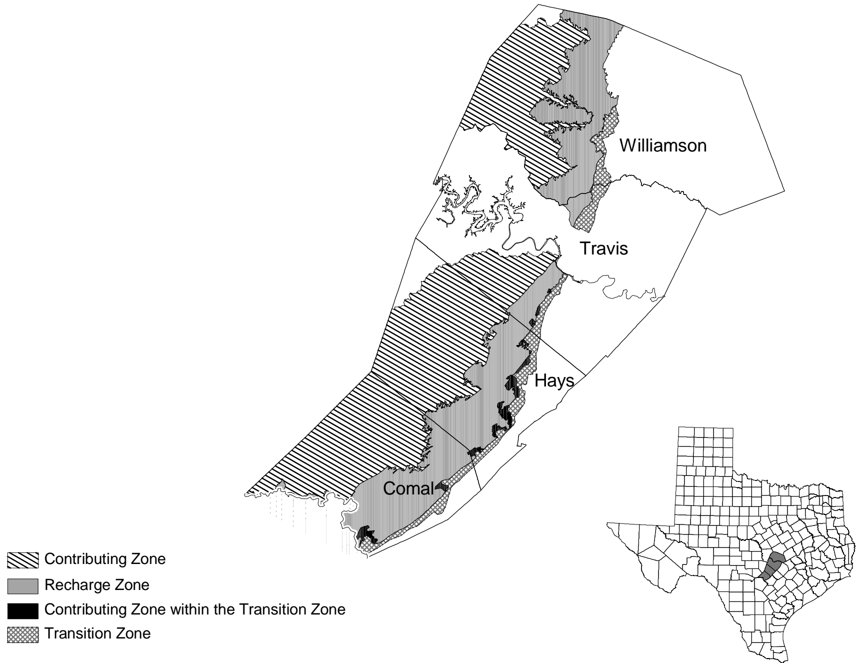
Contributing Zone (Northern Part) for the Edwards Aquifer
